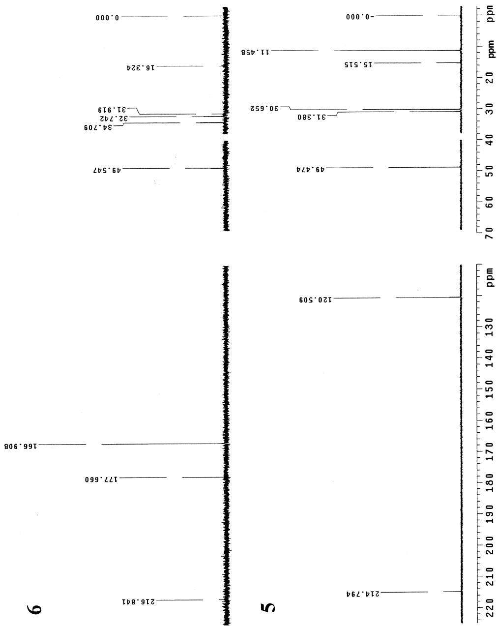
Figure 2. ^{13}\text{C} NMR spectra of 5 and 6 in \text{DMSO-d}_6 . For clarity the solvent peak (39.5 ppm) and the 70-110 ppm interval (with no signals) have been removed.
