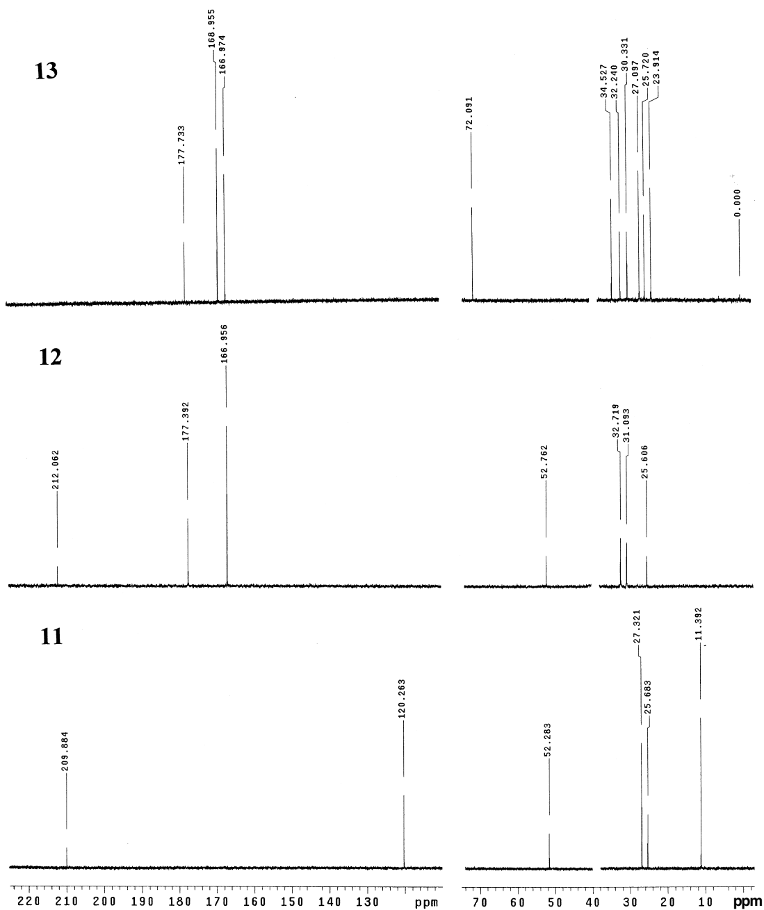
Figure 4. ^{13}\text{C} NMR spectra of 11 , 12 and 13 in \text{DMSO-d}_6 . For clarity the solvent peak (39.5 ppm) and the 75-110 ppm interval (with no signals) have been removed.
