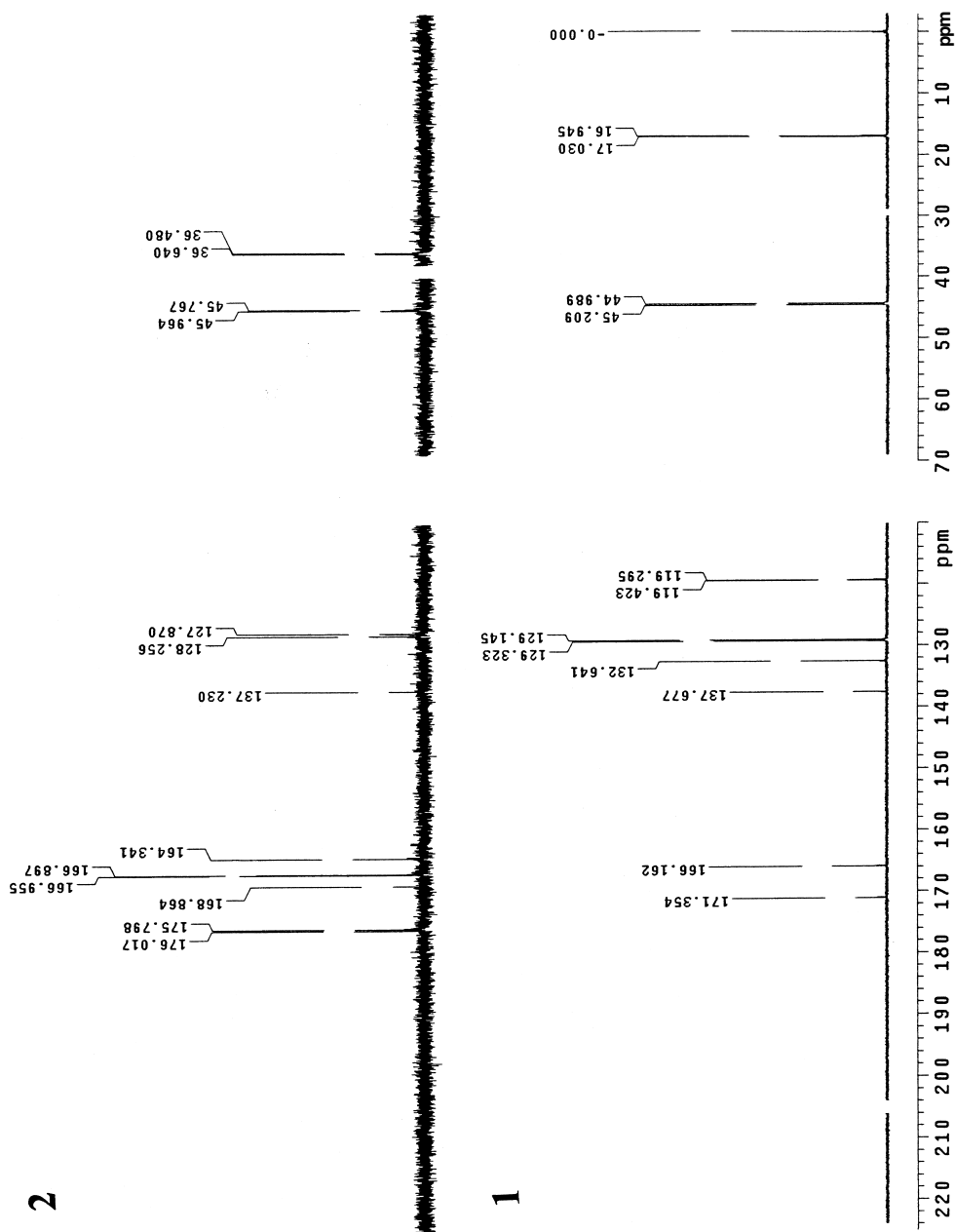
Figure 1. ^{13}\text{C} NMR spectra of 1 in acetone- d_6 and 2 in DMSO- d_6 . For clarity the solvents peaks (acetone- d_6 : 29.8 ppm and 206.0 ppm; DMSO- d_6 : 39.5 ppm) and the 70-110 ppm interval (with no signals) have been removed.
