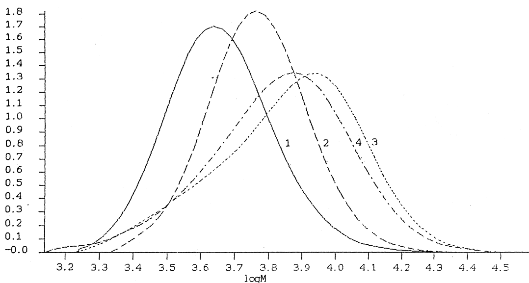
Figure 6. Overlaid differential molecular weight graphs of I G-CN (1), II G-CN (2), III G-CN (3), and IV G-CN (4).
